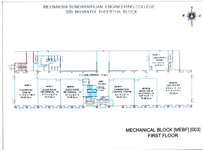
MECHANICAL BLOCK FIRST FLOOR PLAN
