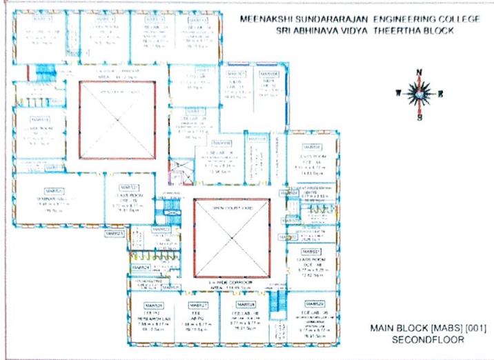
MAIN BLOCK SECOND FLOOR PLAN
