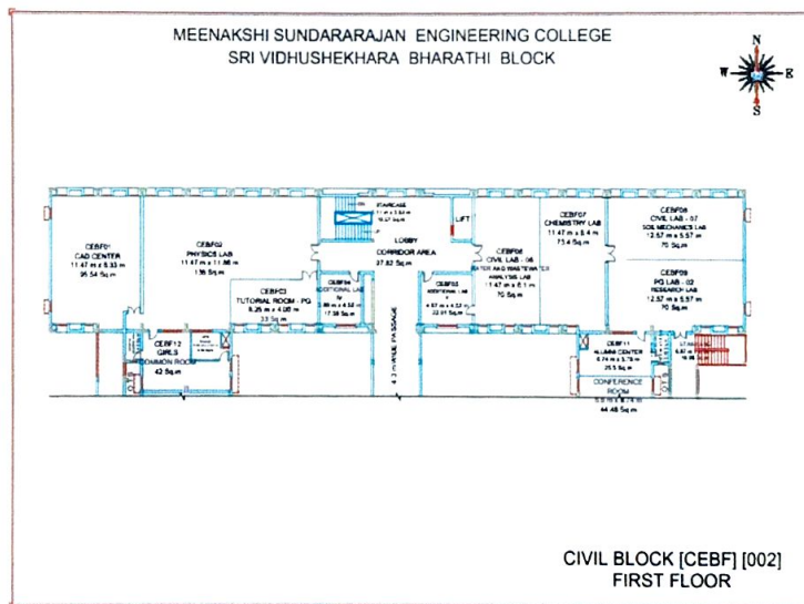
CIVIL BLOCK FIRST FLOOR PLAN
