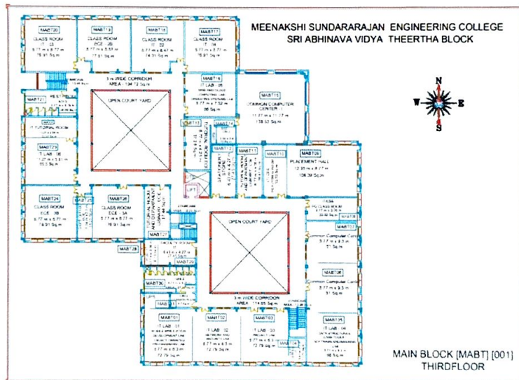
MAIN BLOCK THIRD FLOOR PLAN
