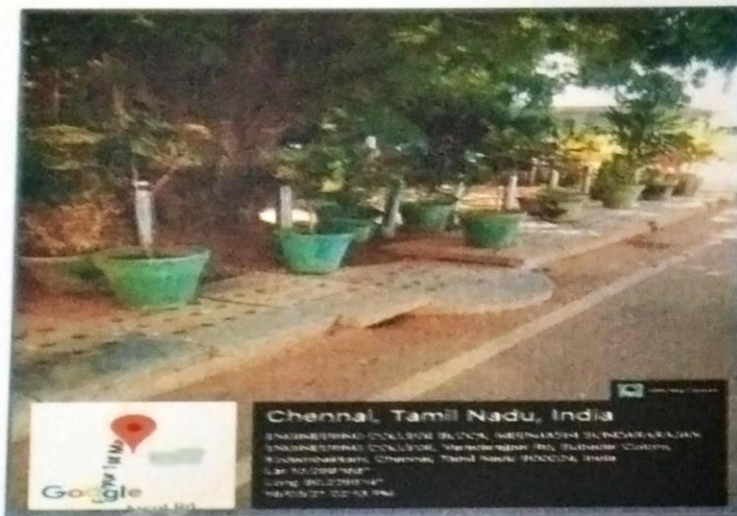
Fig. 1 : RAIN WATER HARVESTING IN THE CAMPUS
