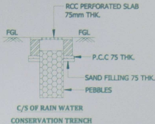
Fig. 1 : Rain water Conservation Trench
